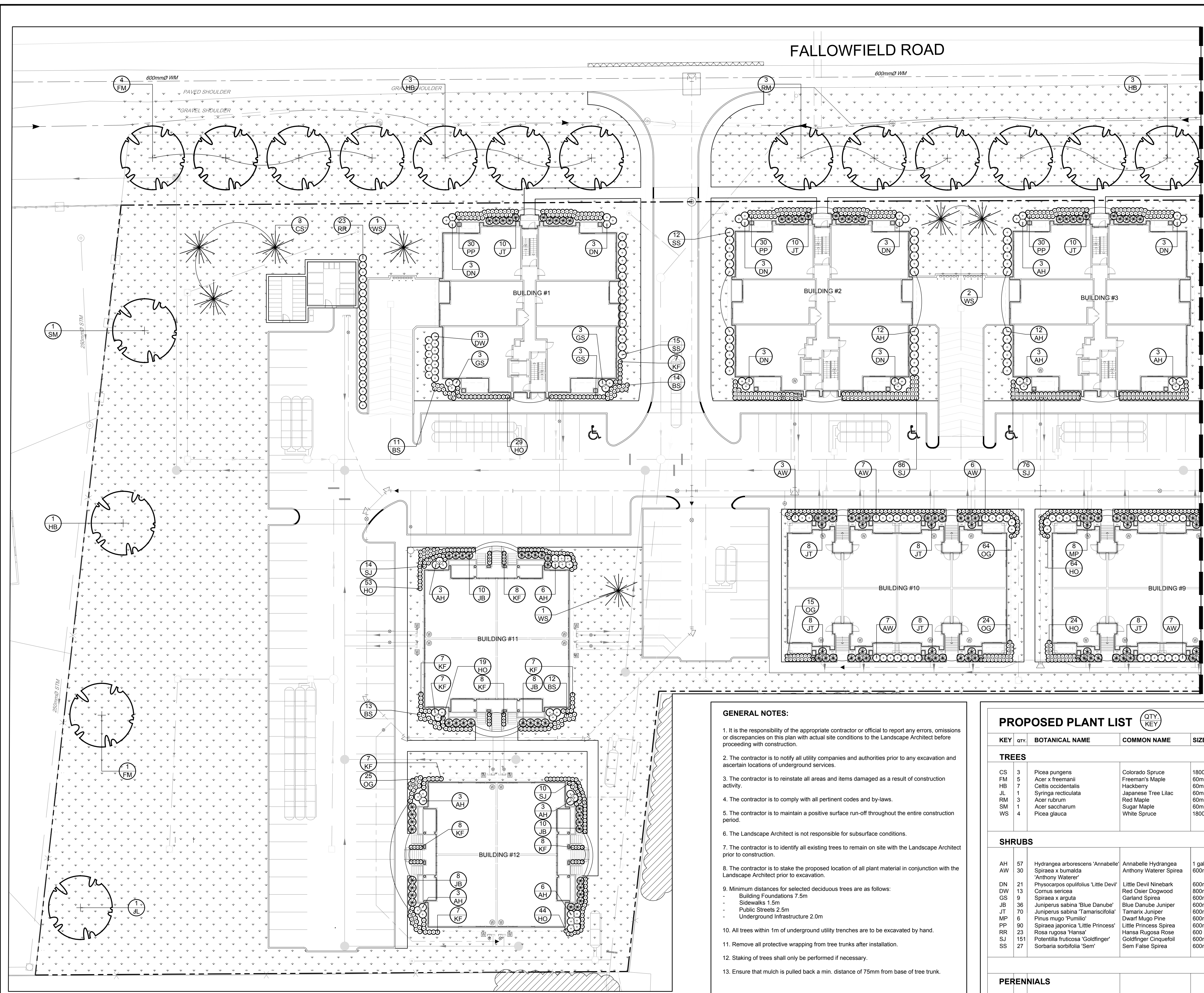
1 LANDSCAPE PLAN L.1 SCALE 1:250
