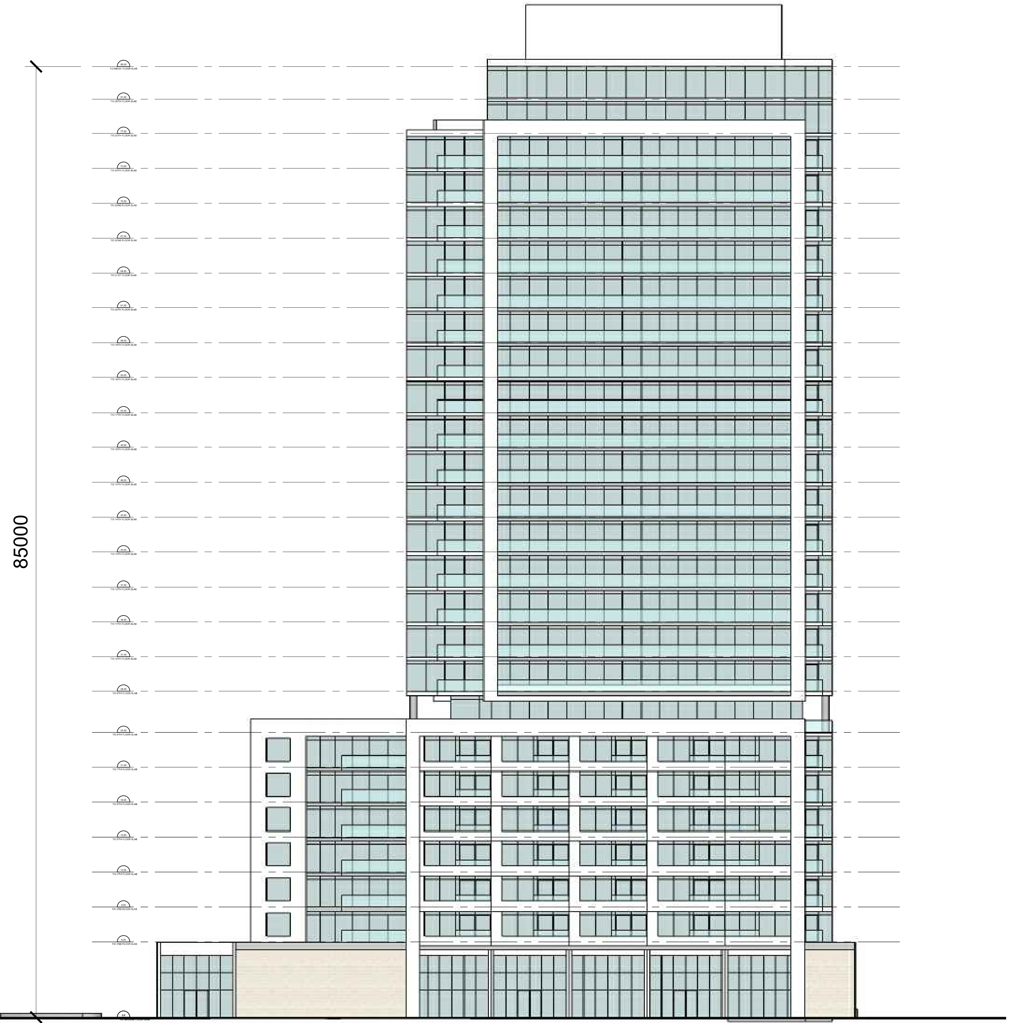
EAST ELEVATION
