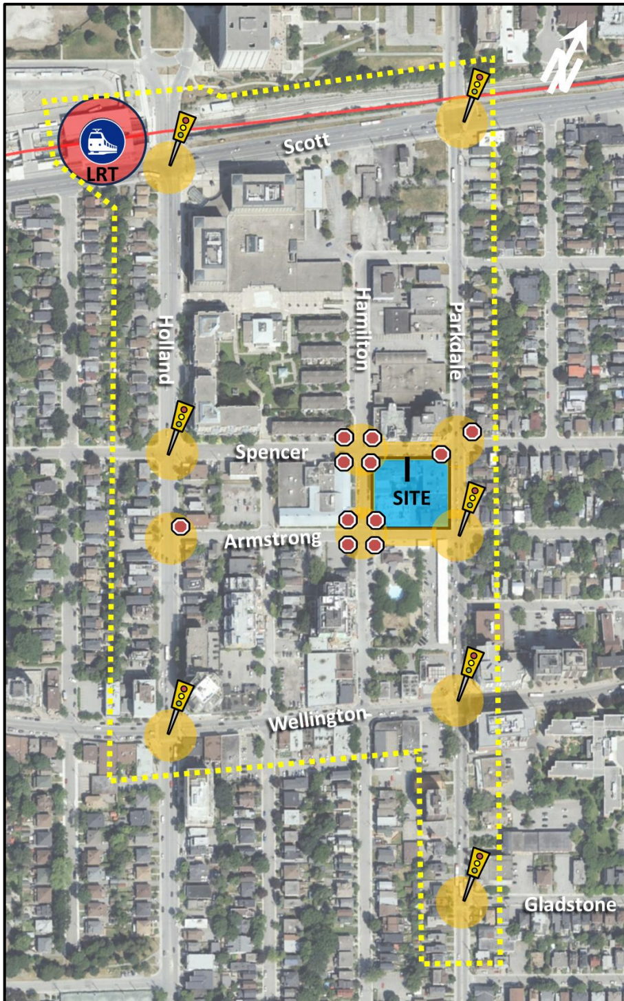
Figure 1: Local Context
