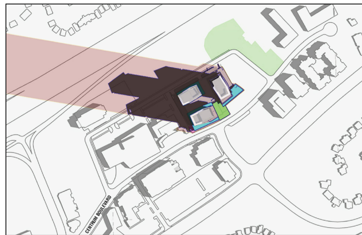
JUNE 21 9 AM
