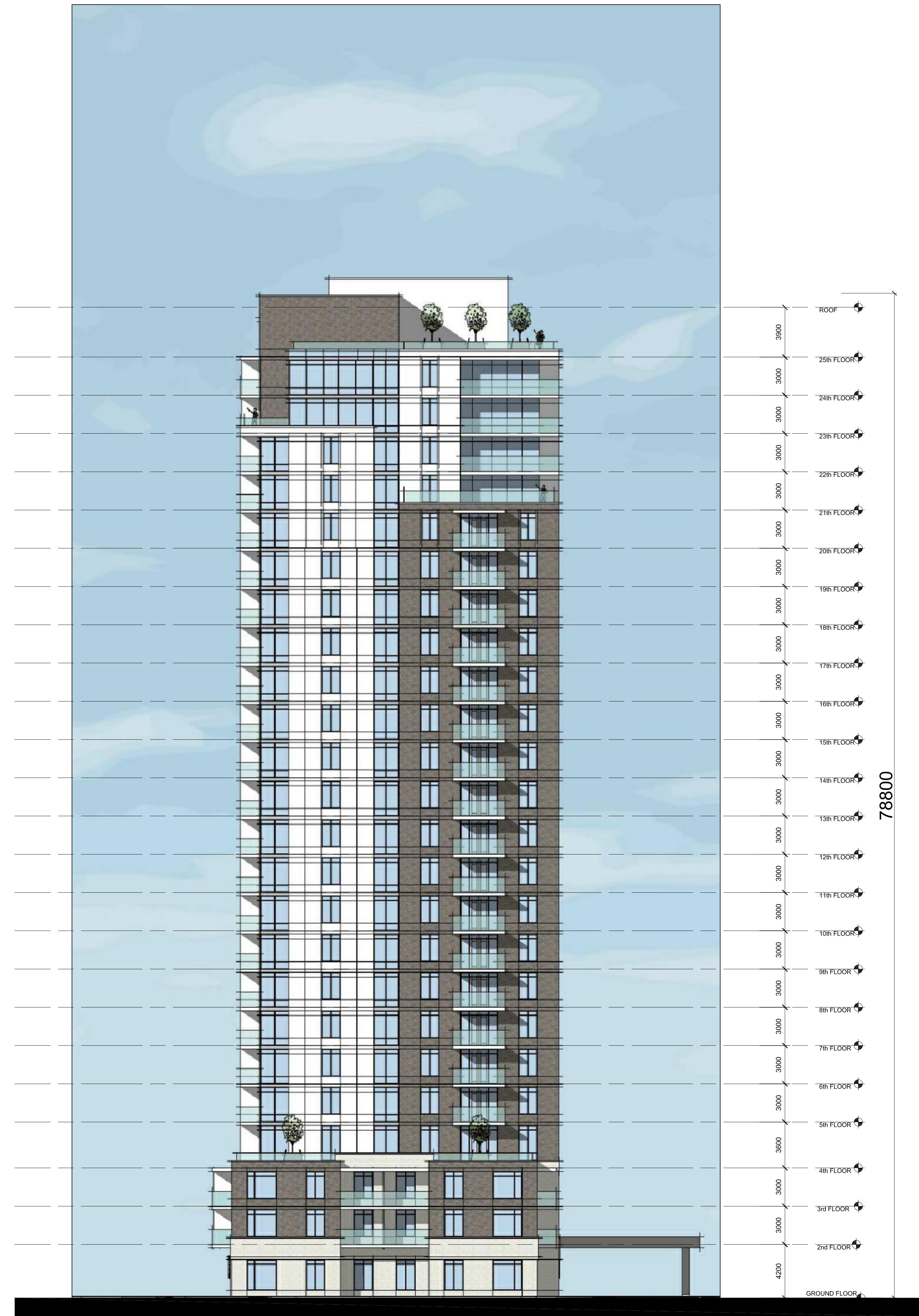
SOUTH ELEVATION
