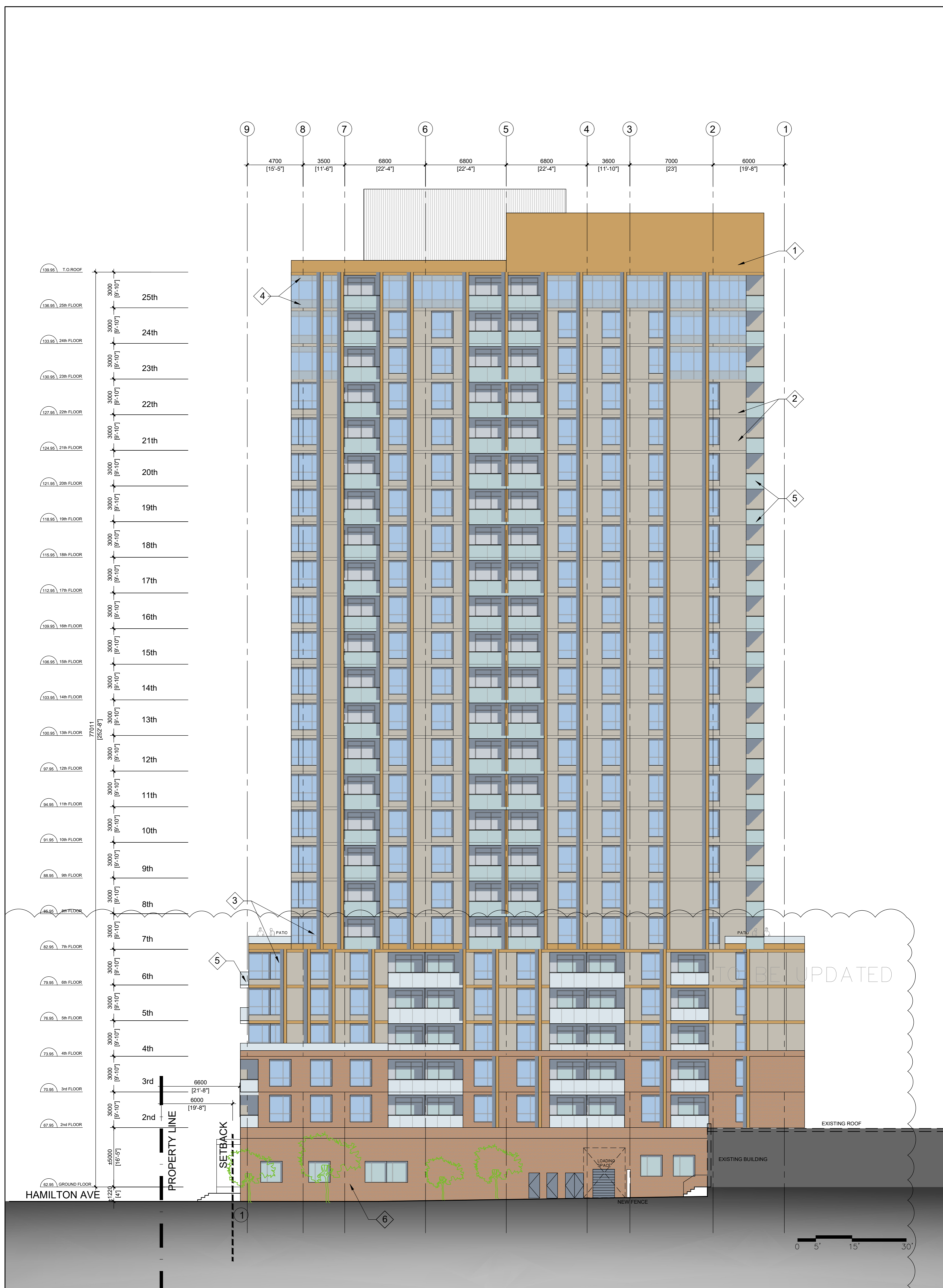
1 NORTH ELEVATION SCALE 1:200
