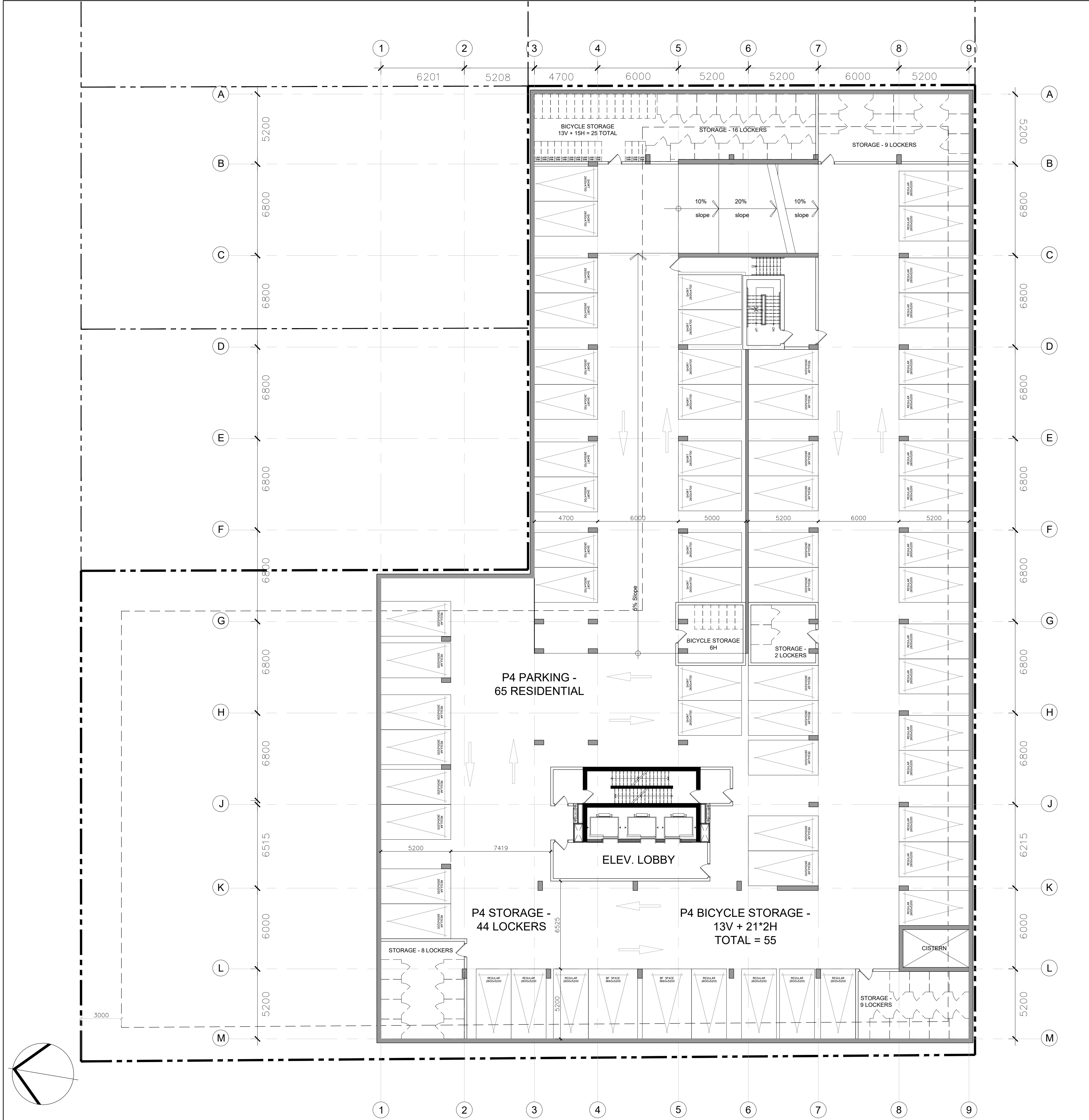
1 LEVEL P4 FLOOR PLAN A2.04 1:150
