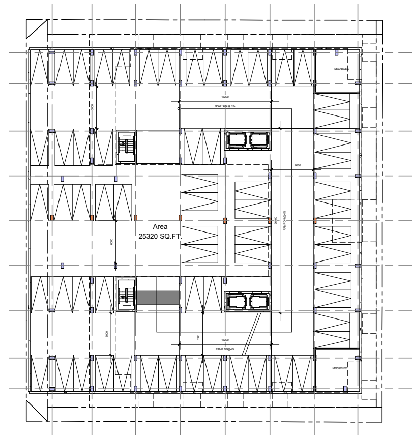
P2 FLOOR PLAN-UP
