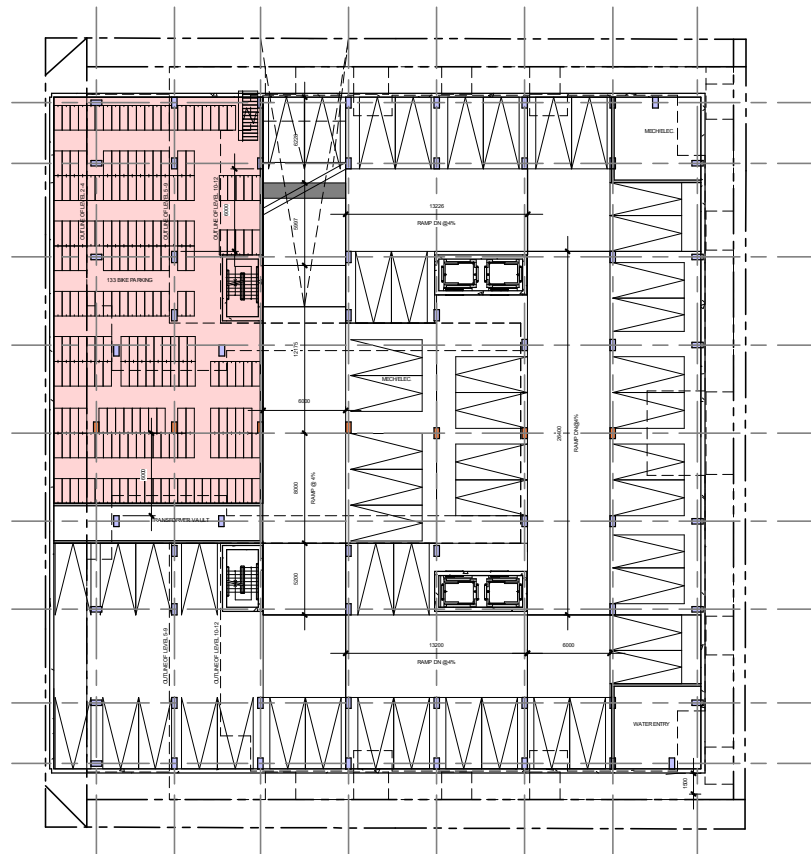
P1 FLOOR PLAN
