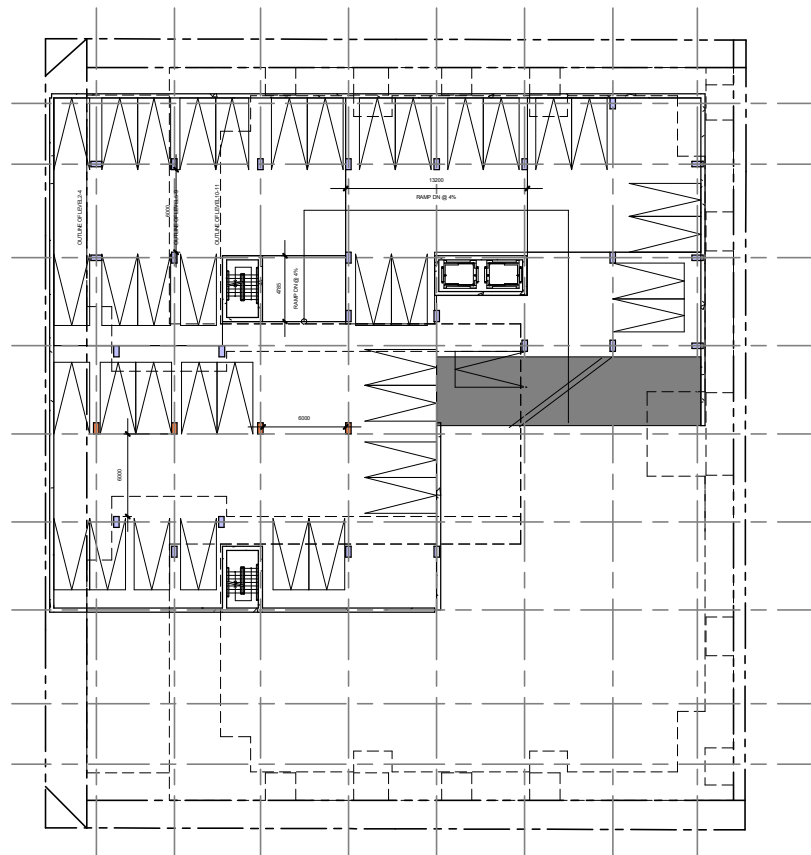
P2 FLOOR PLAN-DN
