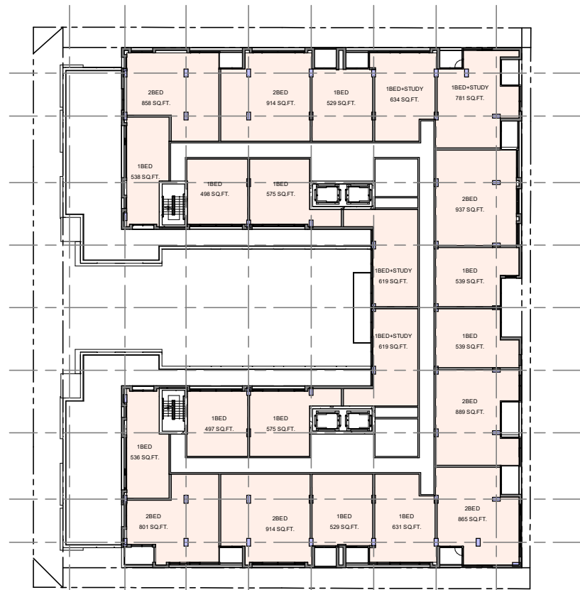
LEVEL 8-9 FLOOR PLAN
