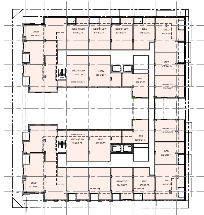
LEVEL 2 FLOOR PLAN
