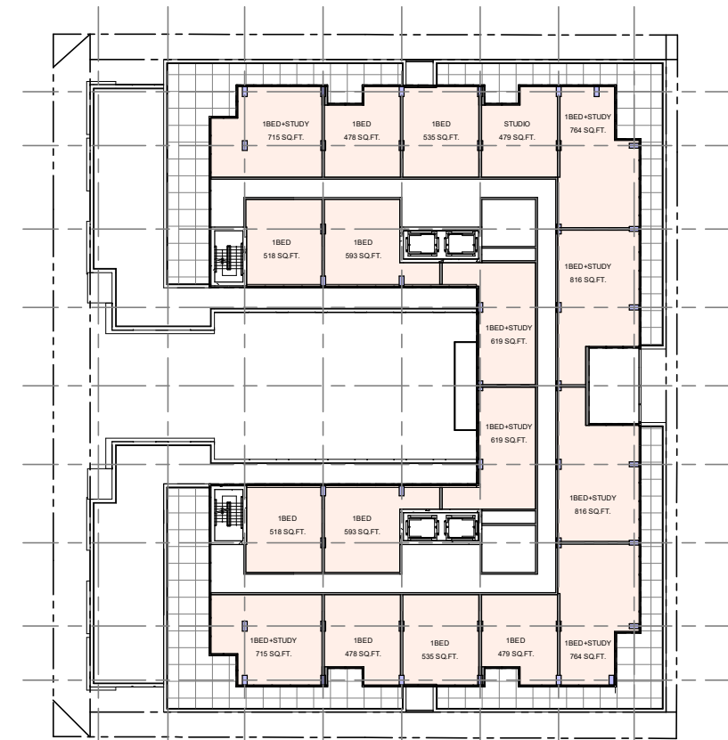
LEVEL 10-11 FLOOR PLAN
