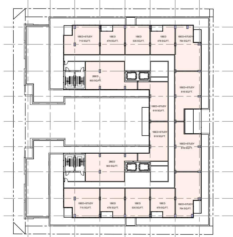
LEVEL 12 FLOOR PLAN
