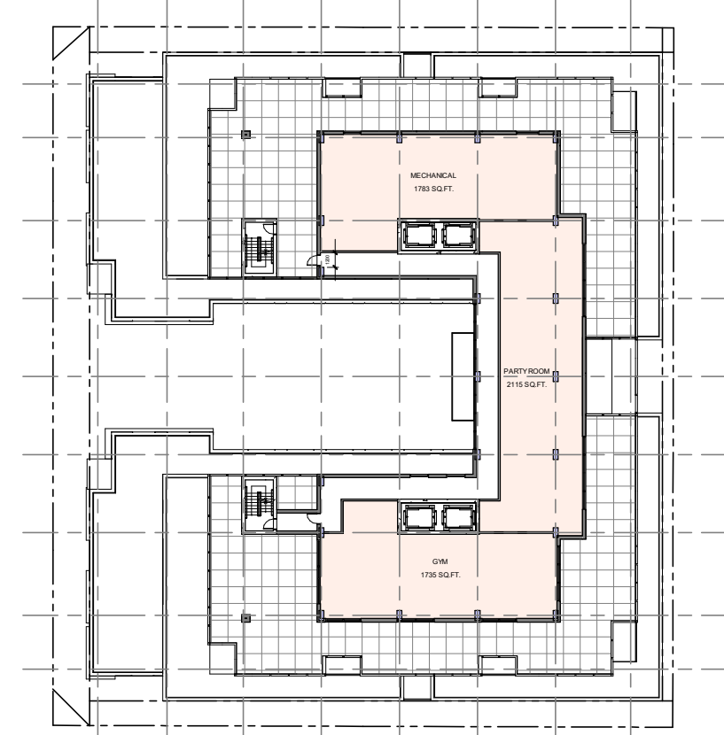
MECHANICAL FLOOR PLAN
