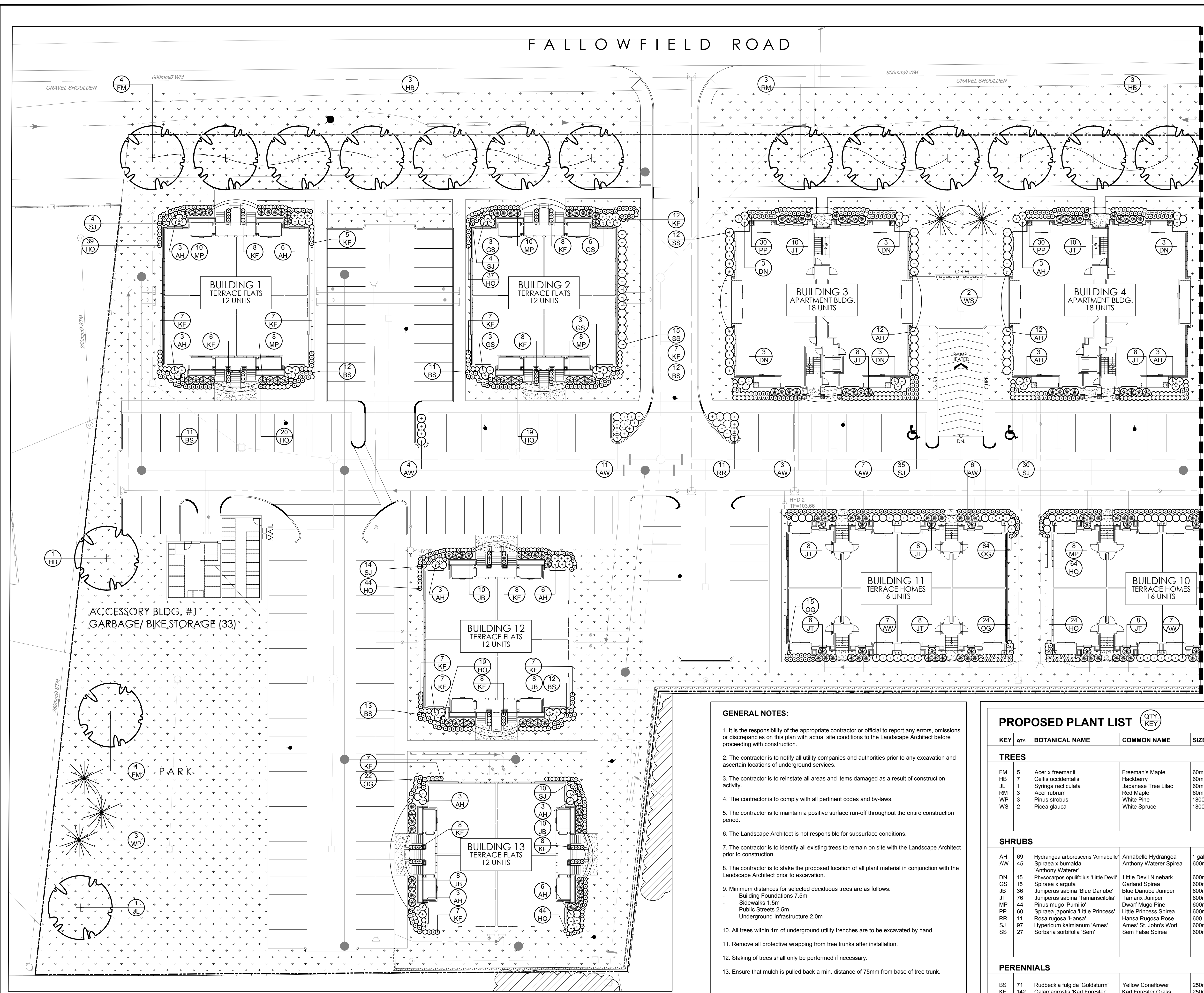
1 LANDSCAPE PLAN SCALE 1:250
